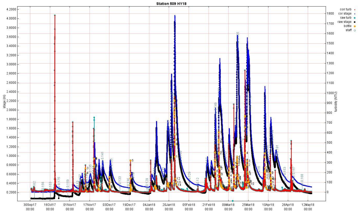
Figure 4: Example Corrected Hydrologic Data Measured at Southfork Elk River (Station 509) for WY 2018.
