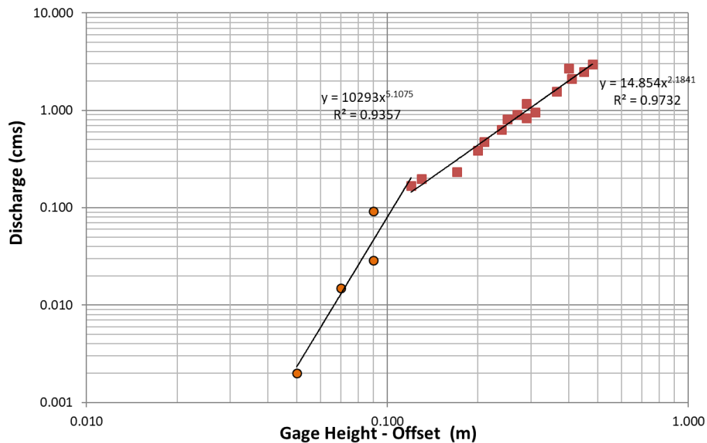
Figure 1: Stage-discharge relationship for Graham Gulch (Station 505), a tributary to freshwater creek. The offset, estimated for the point of zero flow, is 0.05m.
