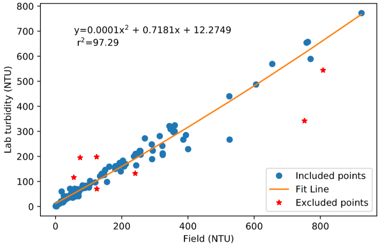
Figure 3: Example Field Turbidity (NTU) vs. Laboratory Turbidity (NTU) for the Mainstem Elk River (Station 509). Note: R^2 = 97.29\% .
