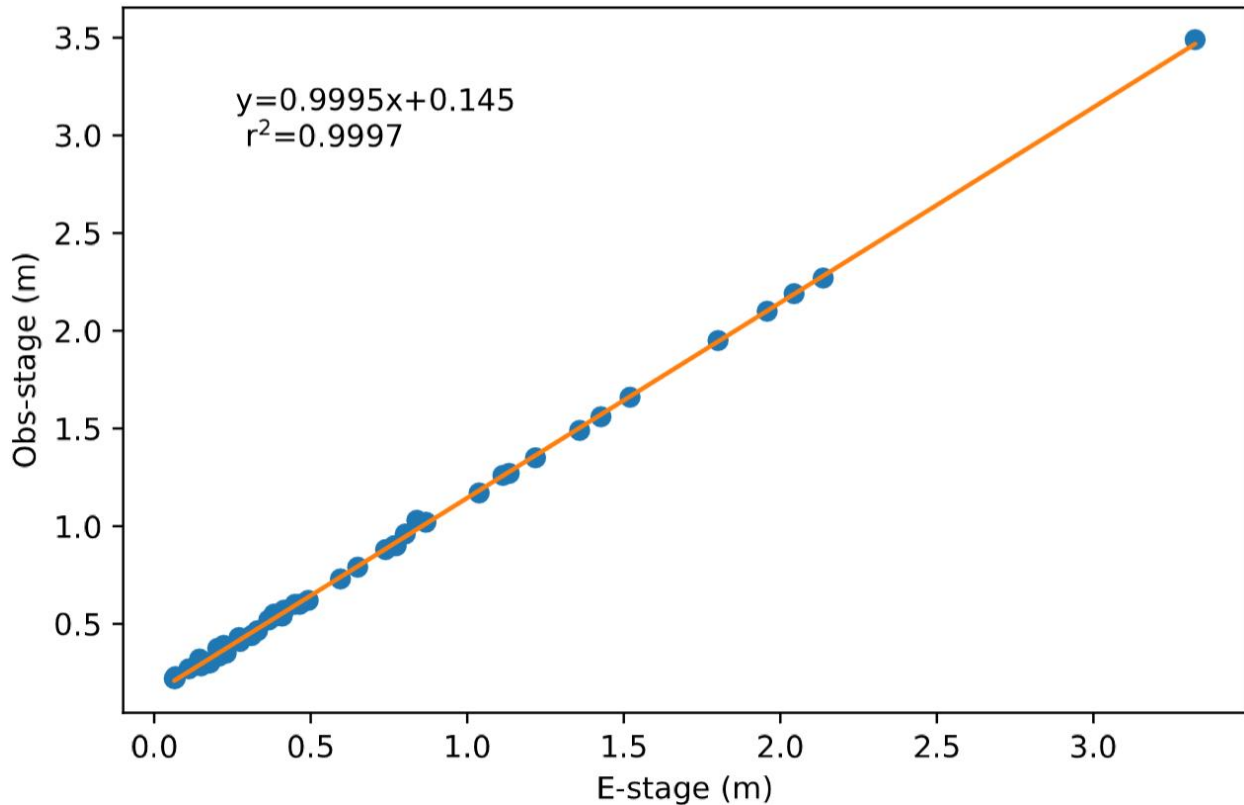
Figure 2: Example Relationship Between 15-Minute Stage (E-Stage) and Observed Stage, Mainstem Elk River (Station 509).
